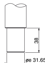
Connection detail
